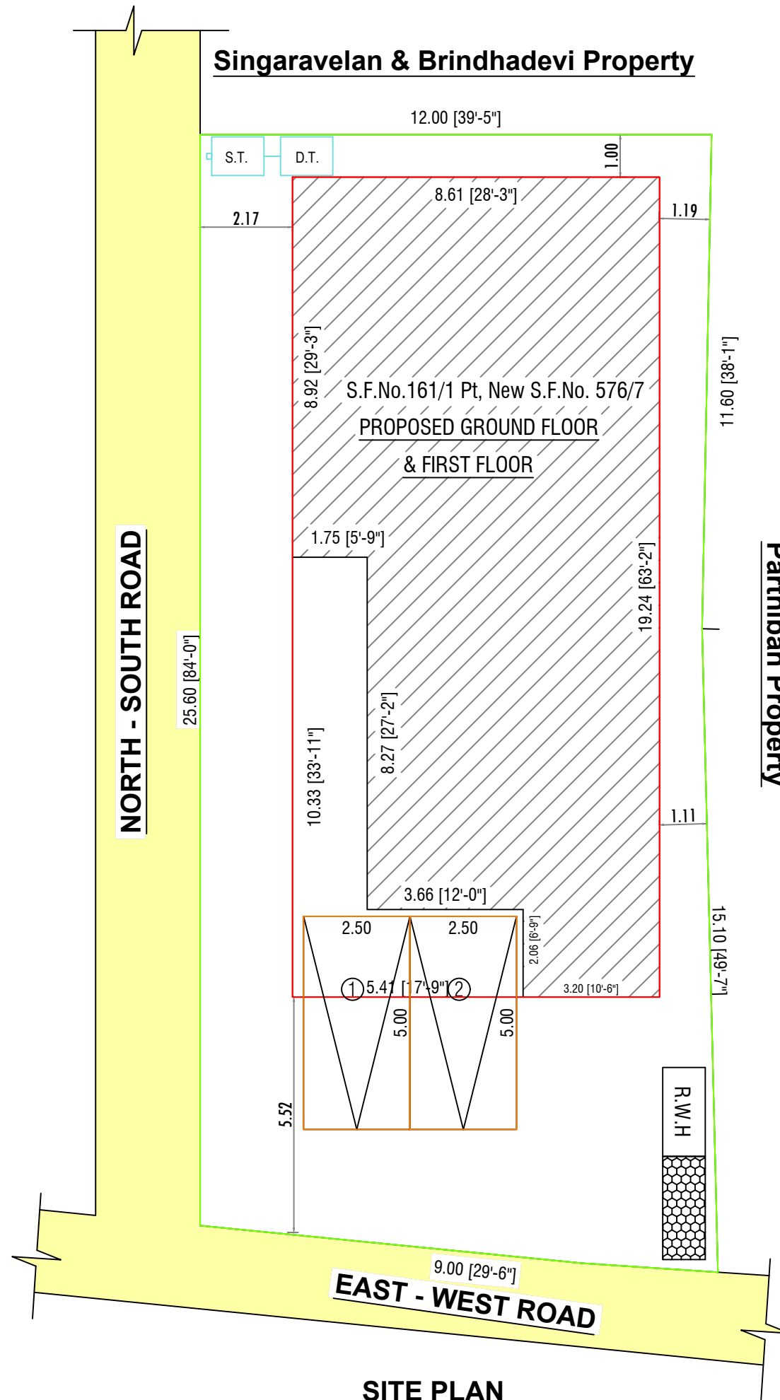
SITE PLAN
