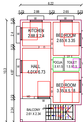
PROPOSED FIRST FLOOR BUILDING
