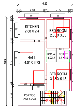
PROPOSED GROUND FOR BUILDING
