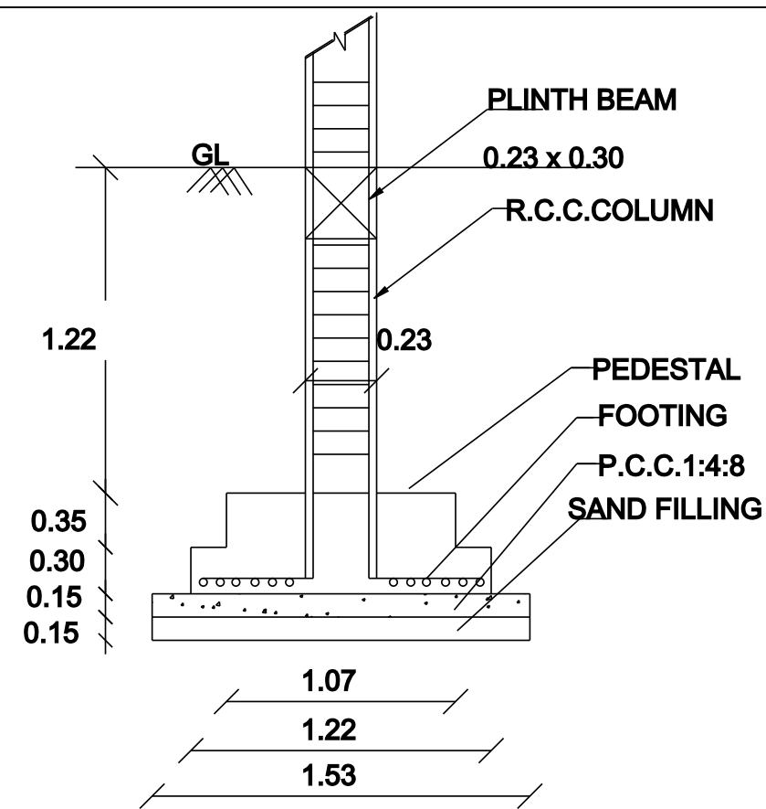
FOUNDATION DETAIL
