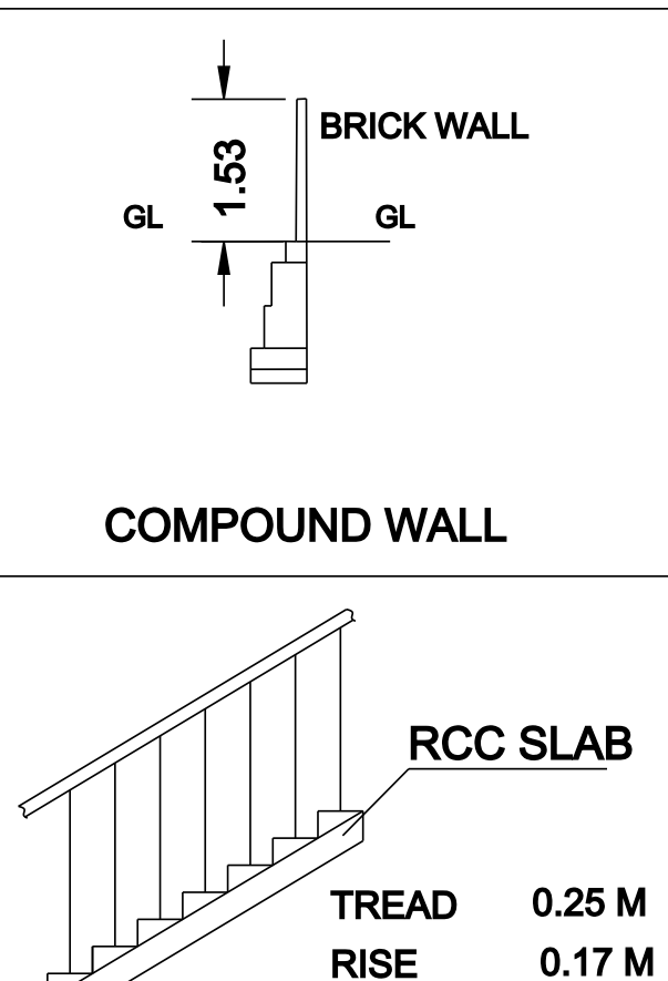
STAIRCASE DETAIL
