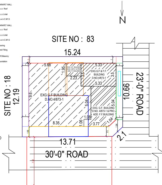
SITE PLAN
