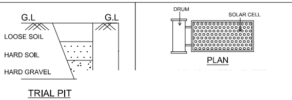
TRIAL PIT
