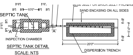
SEPTIC TANK DETAIL SCALE: NTS
