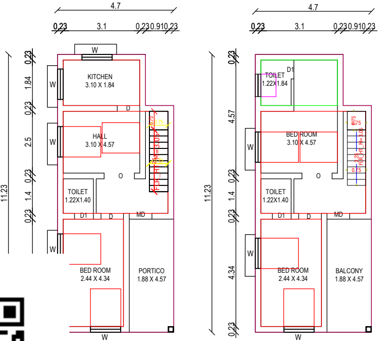
PROPOSED GROUND FLOOR BUILDING
