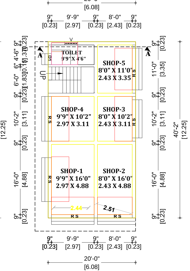
GROUND FLOOR SHOP PLAN
