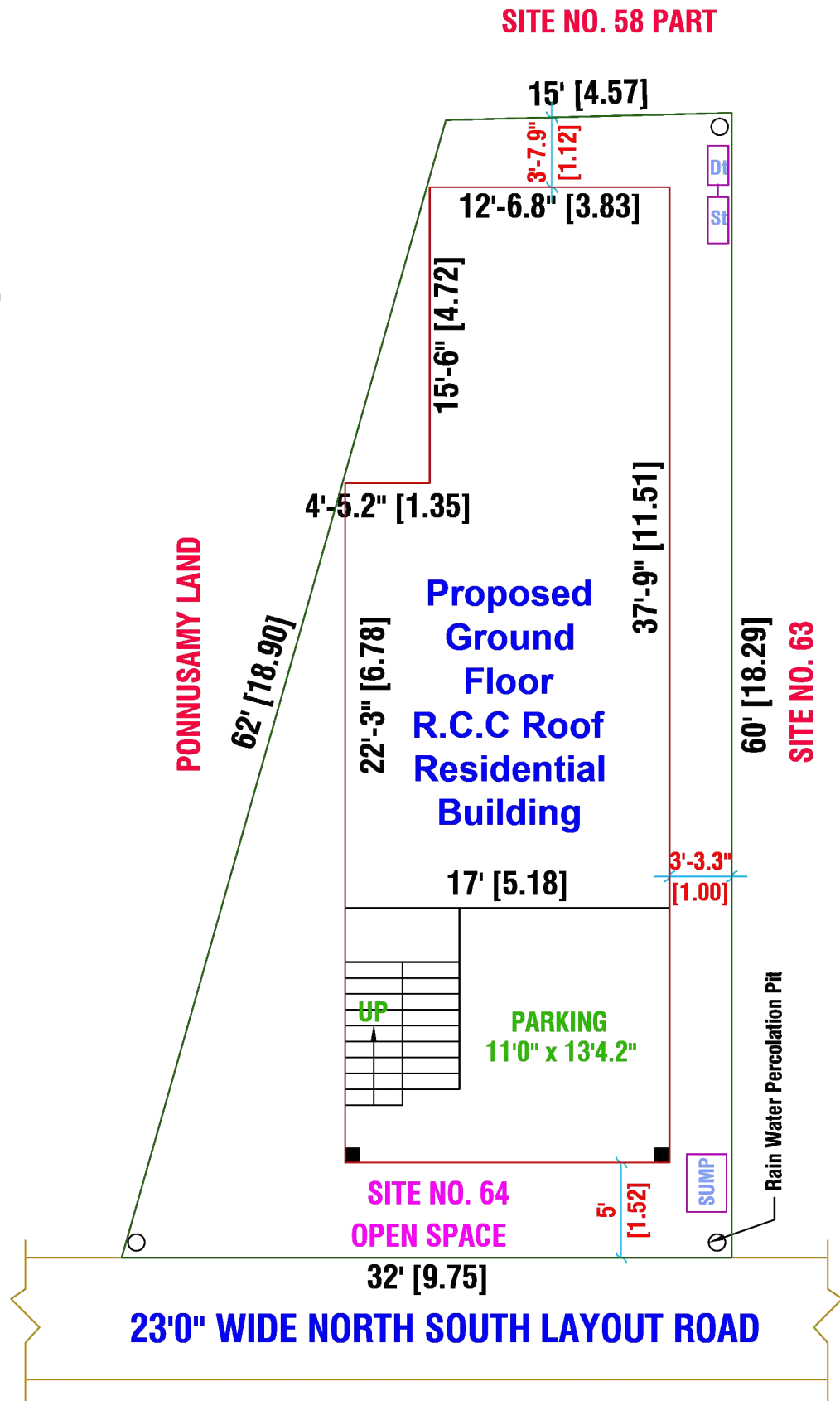
SITE PLAN (SCALE 1" : 8' 0")
