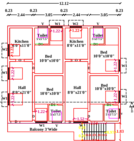
Pro.First Floor Plan
