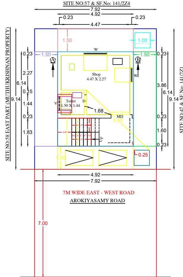
SITE PLAN & EX.APP. GROUND FLOOR PLAN
