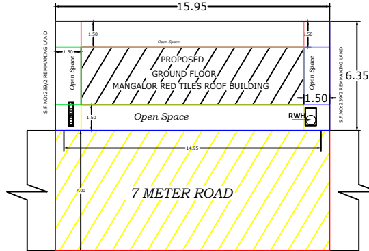
SUPER IMPOSED PLAN SITE PLAN
