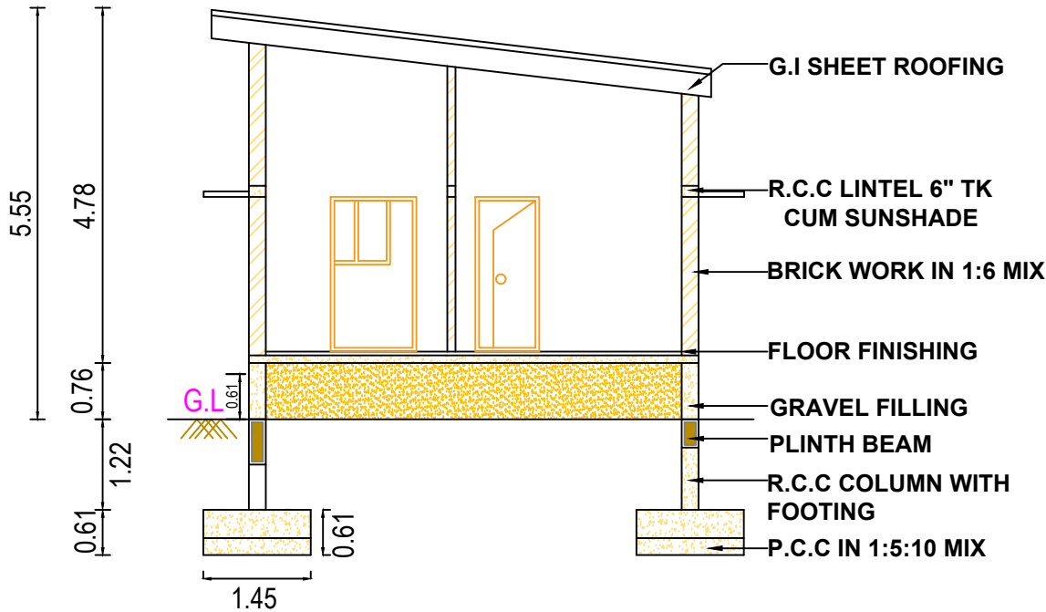
CROSS SECTION AT A-A
