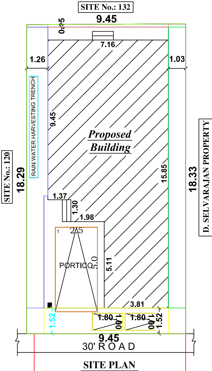
SITE PLAN
