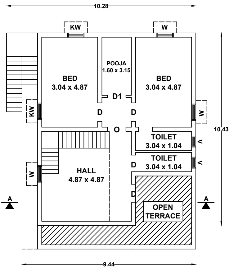
SECOND FLOOR PLAN SCALE - 1' 0" = 8' 0"
