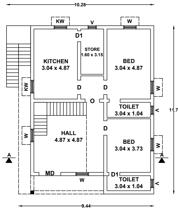
FIRST FLOOR PLAN SCALE - 1' 0" = 8' 0"
