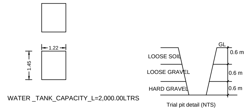
Trial pit detail (NTS)
