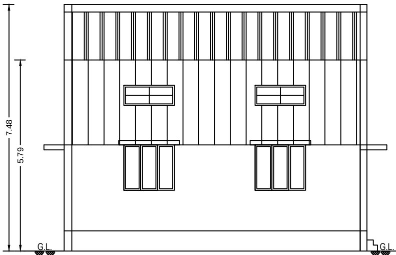
Elevation-South Side
