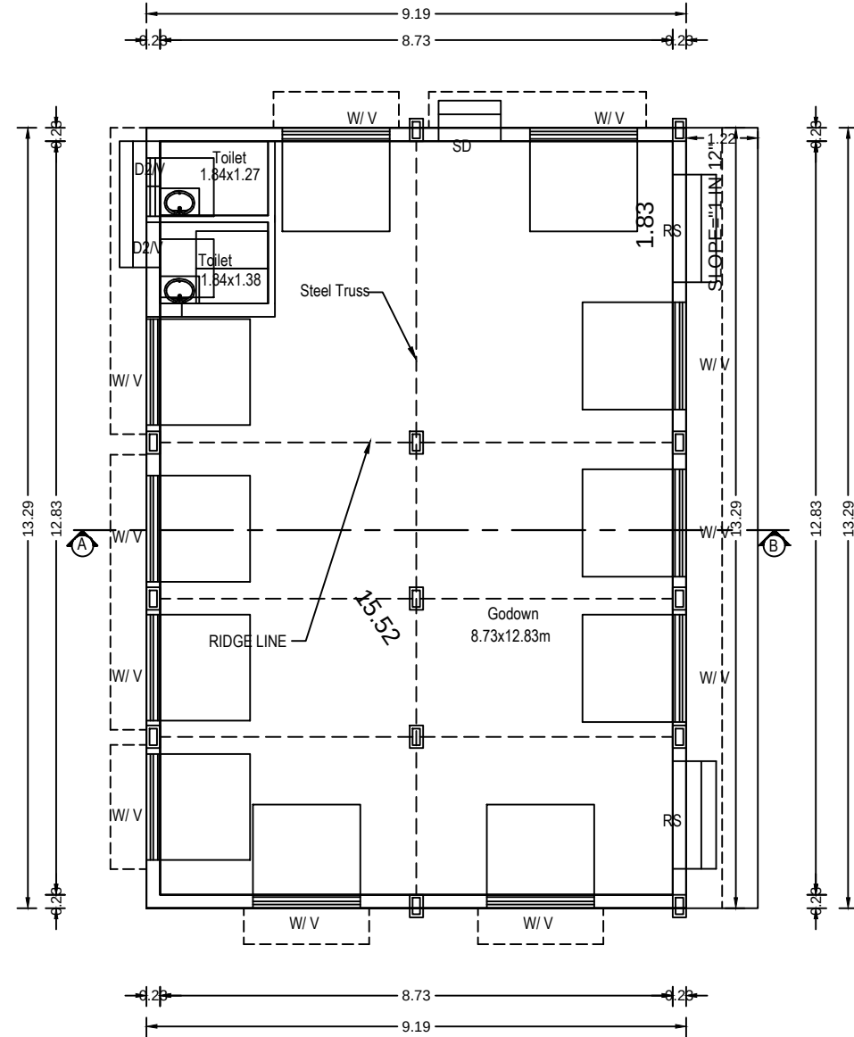
SCALE 1:100 GROUND FLOOR PLAN
