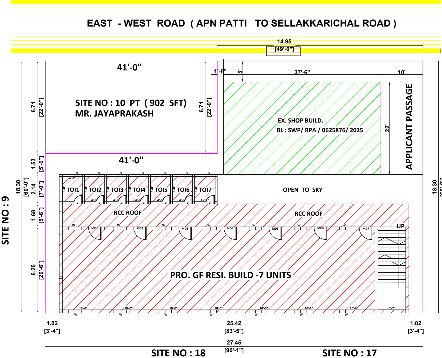
SITE PLAN ( SITE NO : 10 PART AND 11 )
