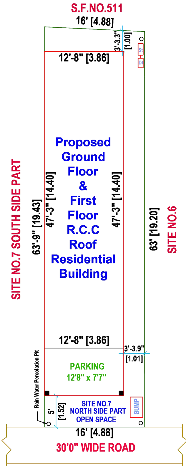
SITE PLAN
