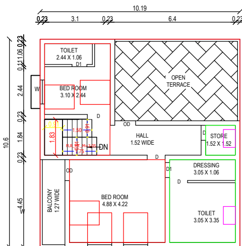
PROPOSED FIRST FLOOR BUILDING
