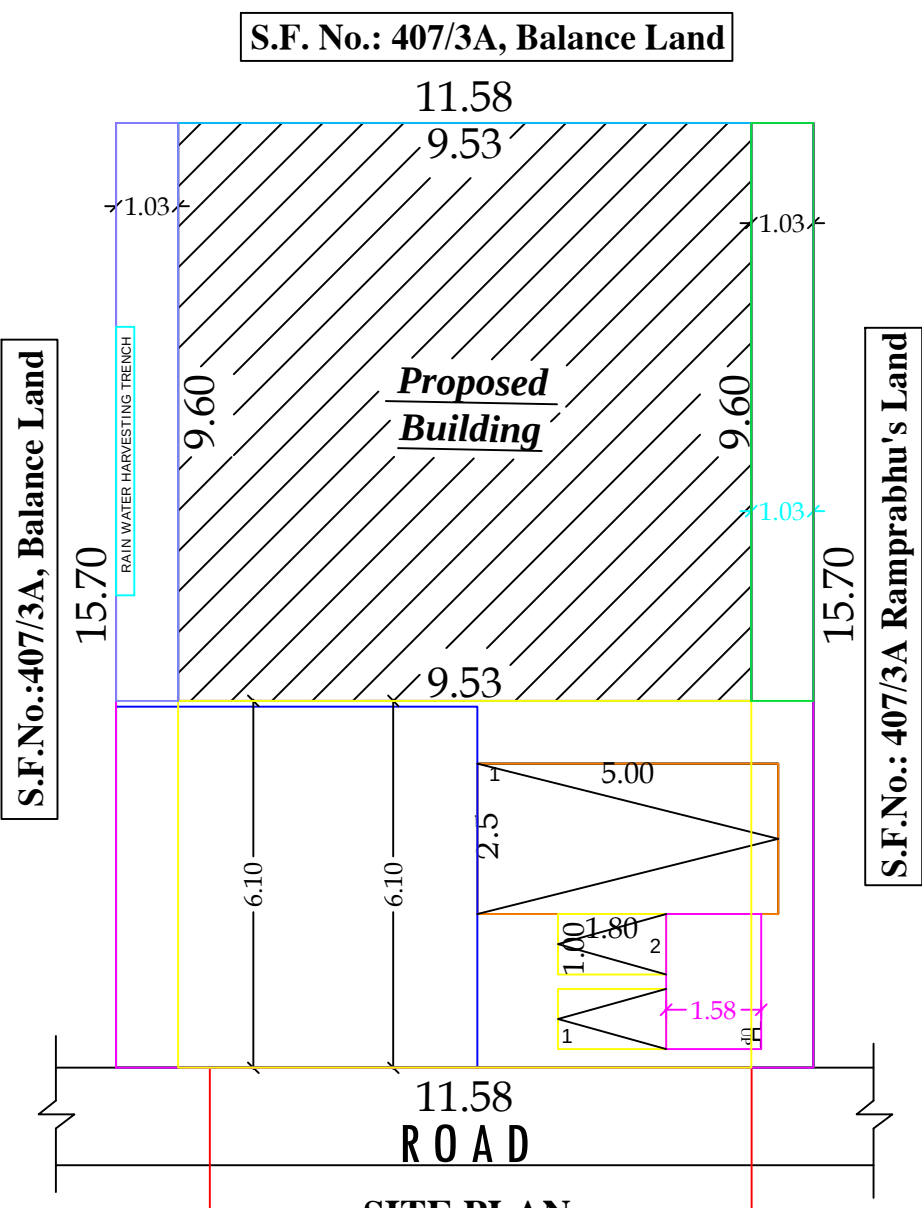
SITE PLAN
