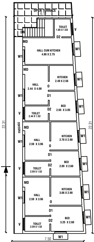
ADDITIONAL PROPOSED FIRST FLOOR PLAN
