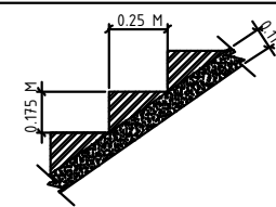
STAIRCASE DETAILS: WIDTH : 1.00 M RAISER : 0.175 M
