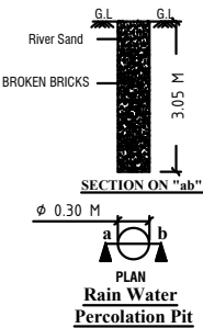
PLAN Rain Water Percolation Pit
