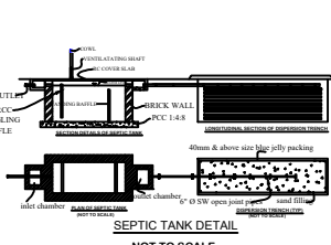
SEPTIC TANK DETAIL
