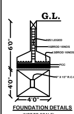
FOUNDATION DETAILS
