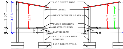
CROSS SECTION A-A
