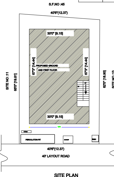
SITE PLAN
