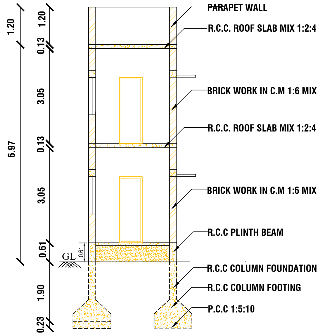
CROSS SECTION AT A-A
