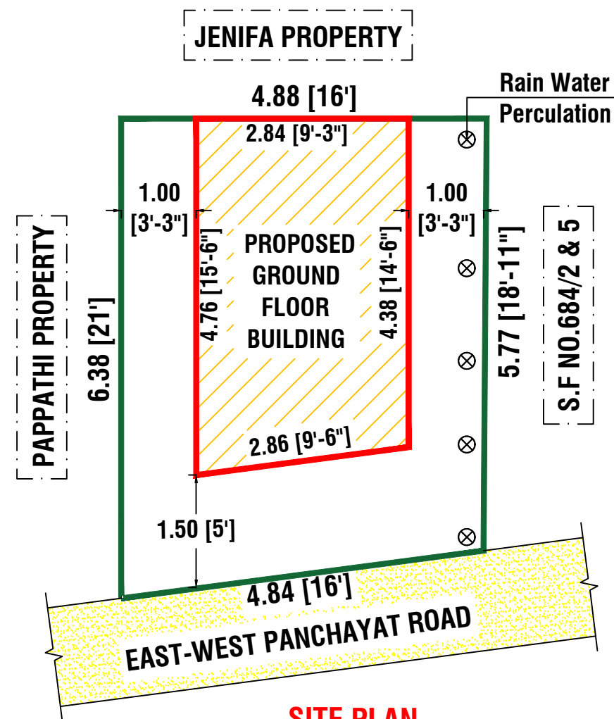
SITE PLAN
