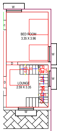
PROPOSED FIRST FLOOR BUILDING
