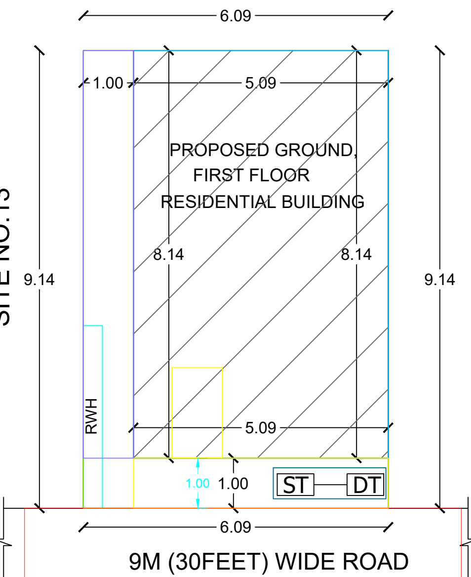
SITE PLAN
