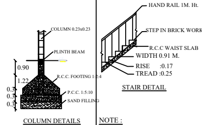
COLUMN DETAILS
