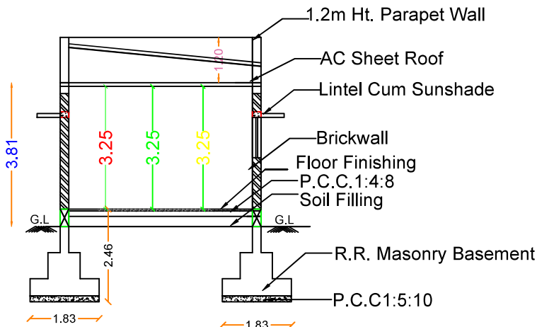
SECTION A-A OWNER'S EXTRA LAND
