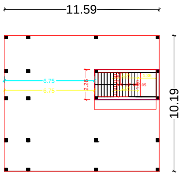
STILT FLOOR PLAN
