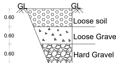
TRIAL PIT (Not To Scale)
