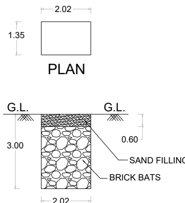
SECTION Not to Scale
