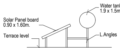
SOLAR WATER HEATING SYSTEM (NOT TO SCALE)
