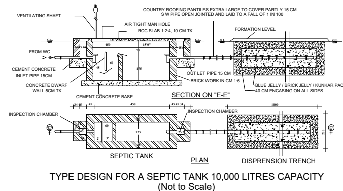
TYPE DESIGN FOR A SEPTIC TANK 10,000 LITRES CAPACITY (Not to Scale)
