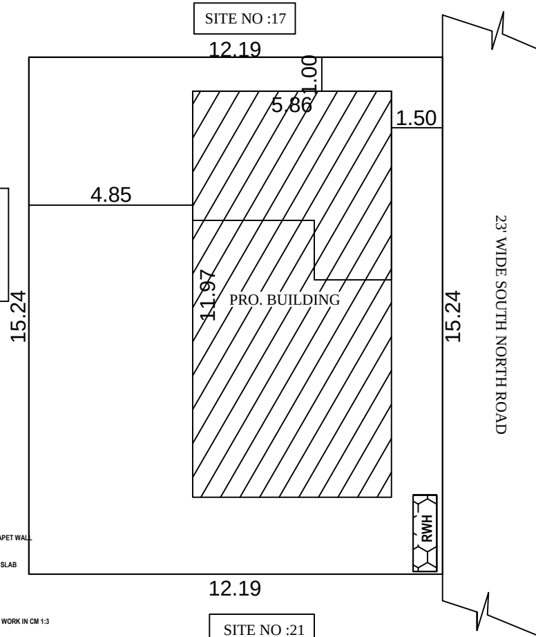
SITE PLAN
