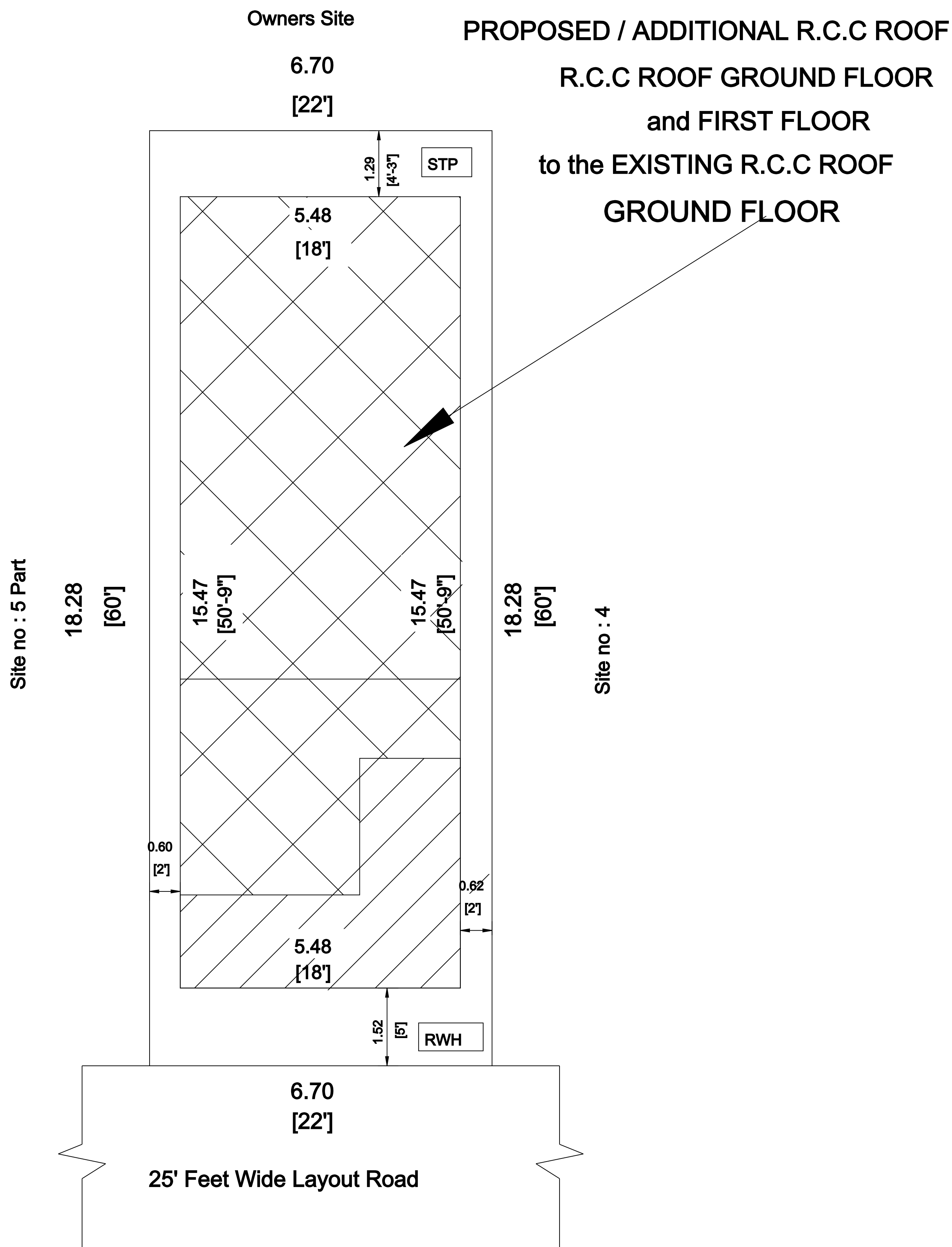
SITE PLAN
