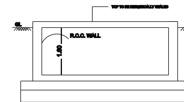
RWHS_SECTION = RWH_SECTION (SAMPLE) RWHS_CAPACITY_L = 2000LTRS
