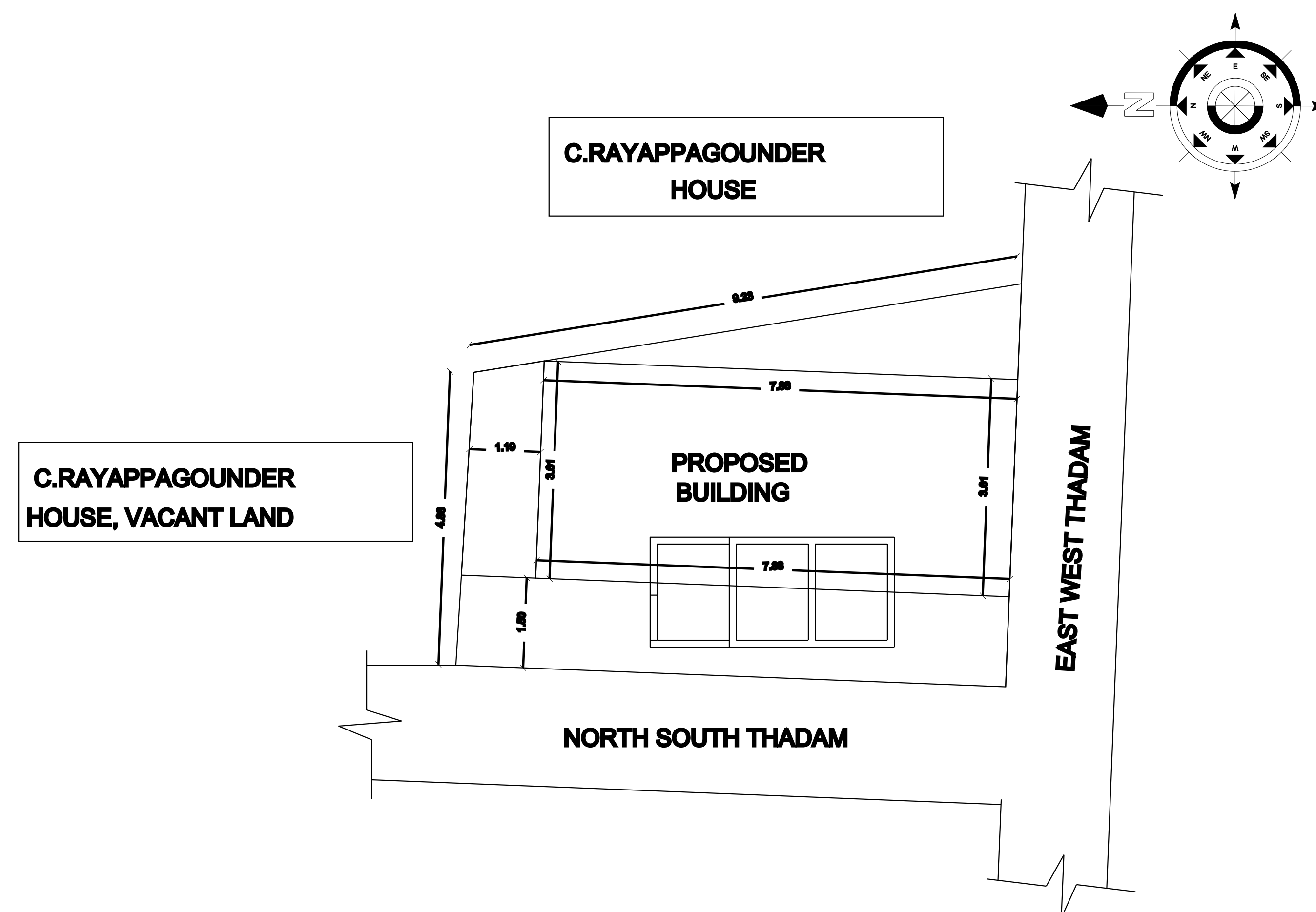
SITE PLAN
