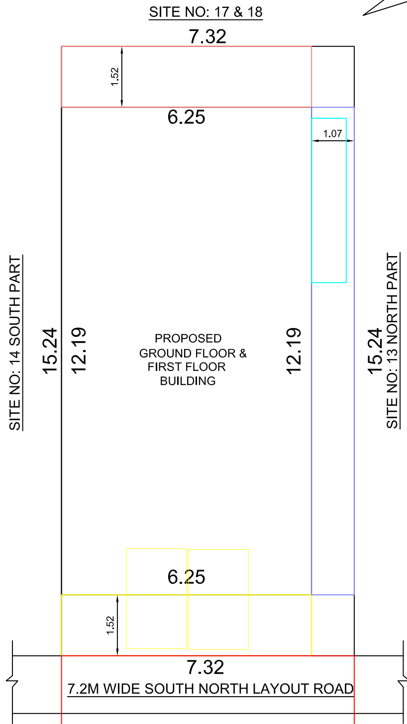
SITE PLAN
