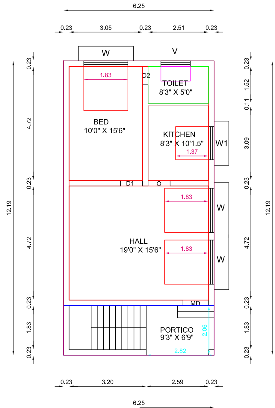
FLOOR PLAN
