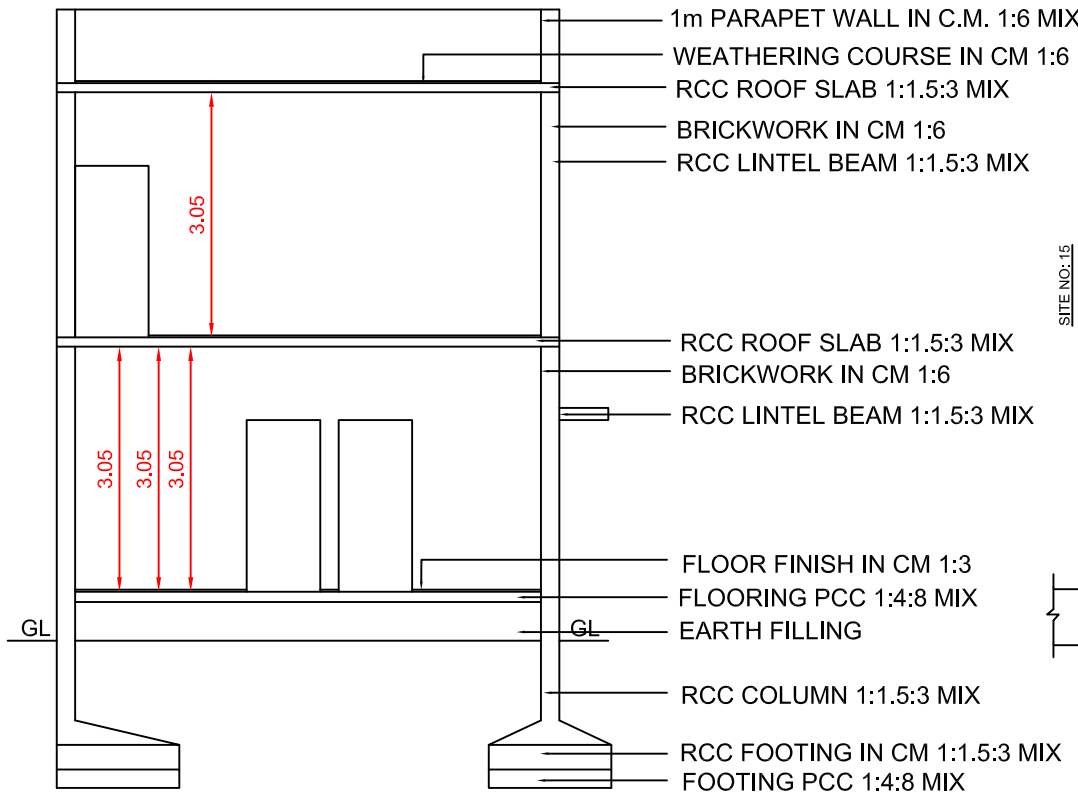
CROSS SECTION ON XY
