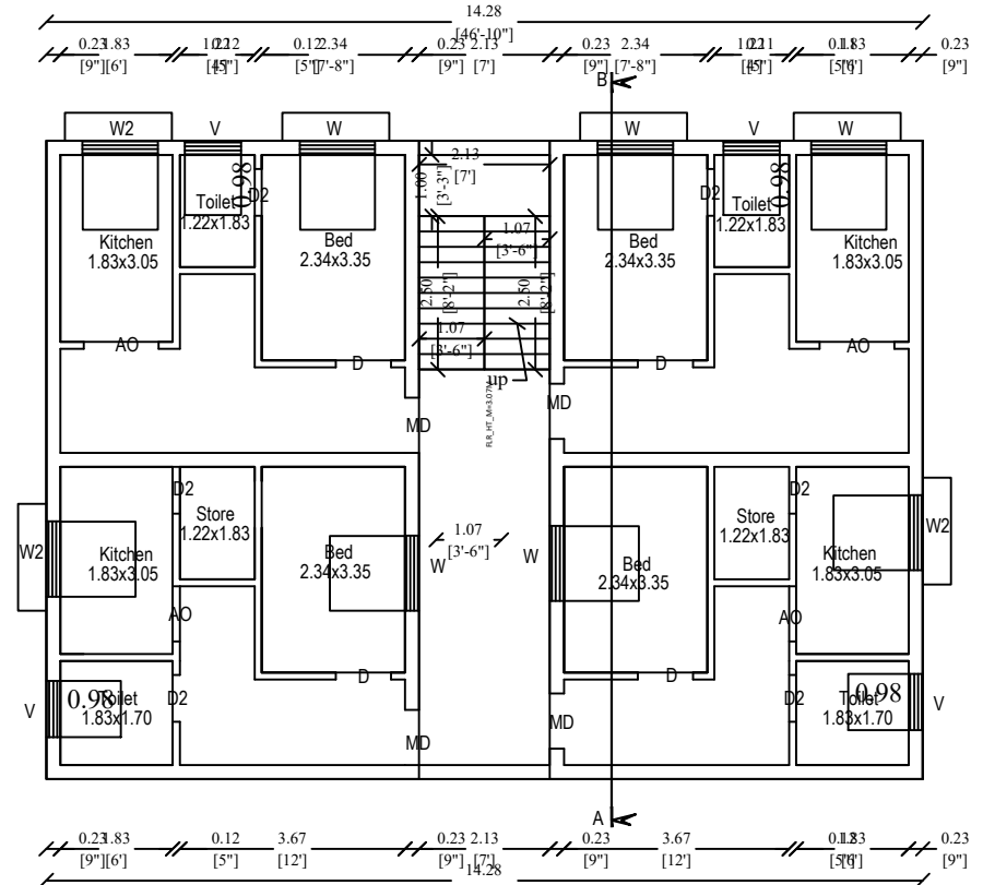
Plan Scale 1:100 Pro.First floor
