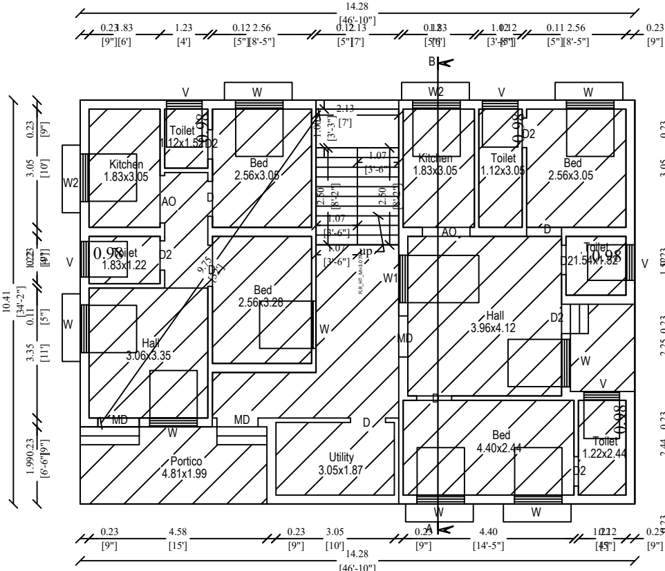
Plan Scale 1:100 Exg. Ground floor
