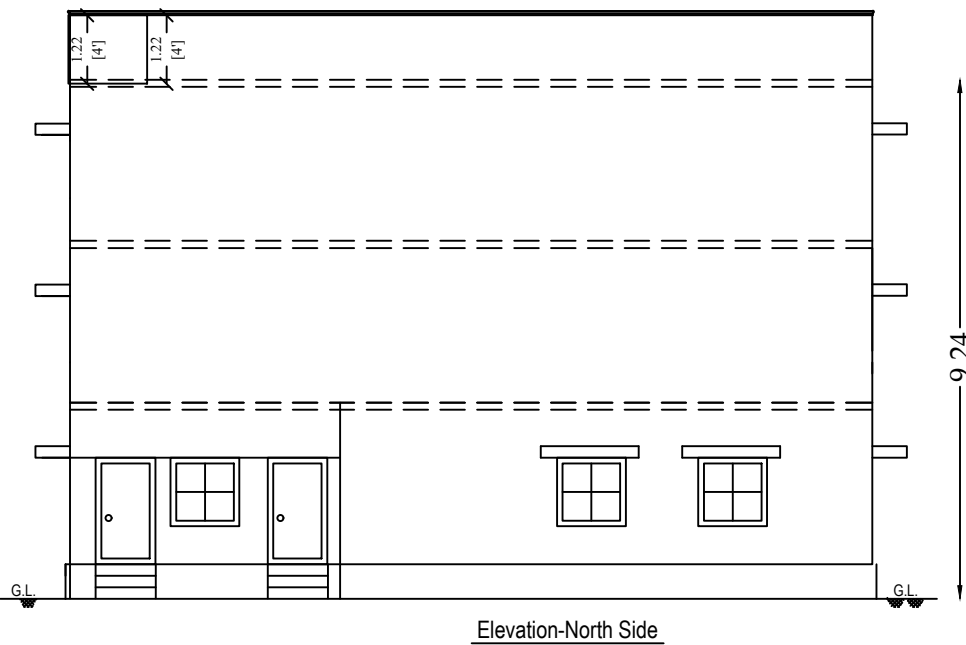
Elevation-North Side
