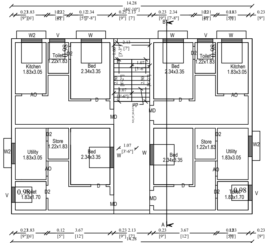
Plan Scale 1:100 Pro.Second floor
