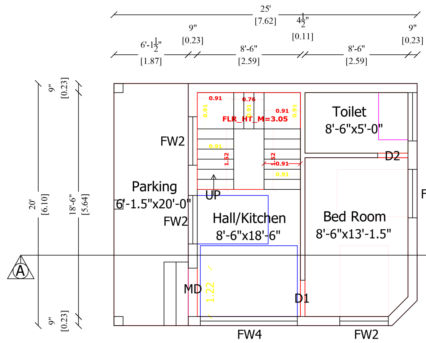
2D FLOOR PLAN
