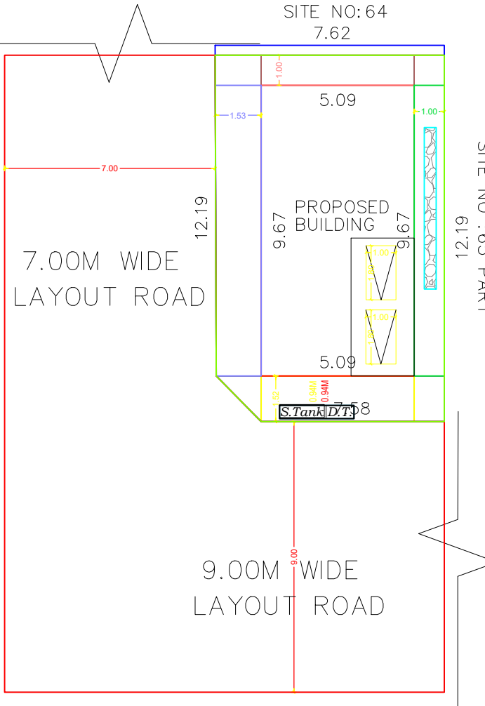
SITE PLAN
