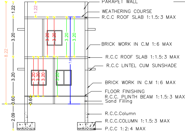
SECTION
