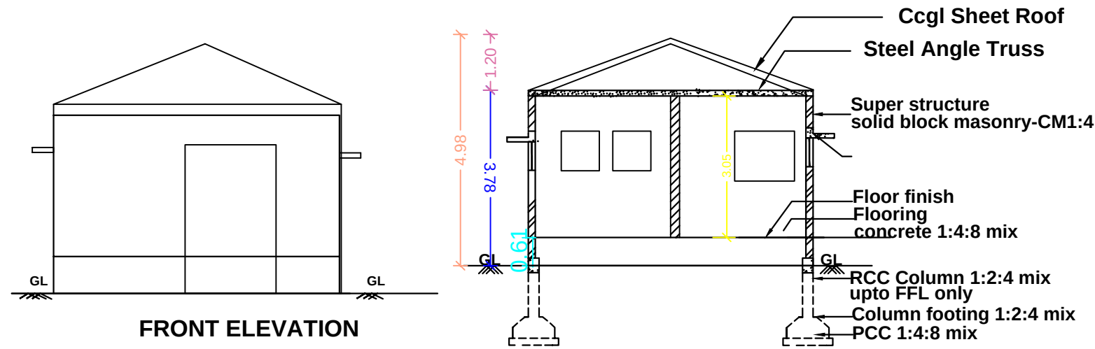
SECTION ELEVATION
