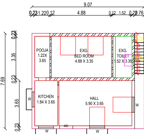
EXG.& PRO.ADDI.GROUND FLOOR PLAN D.NO:1/277
