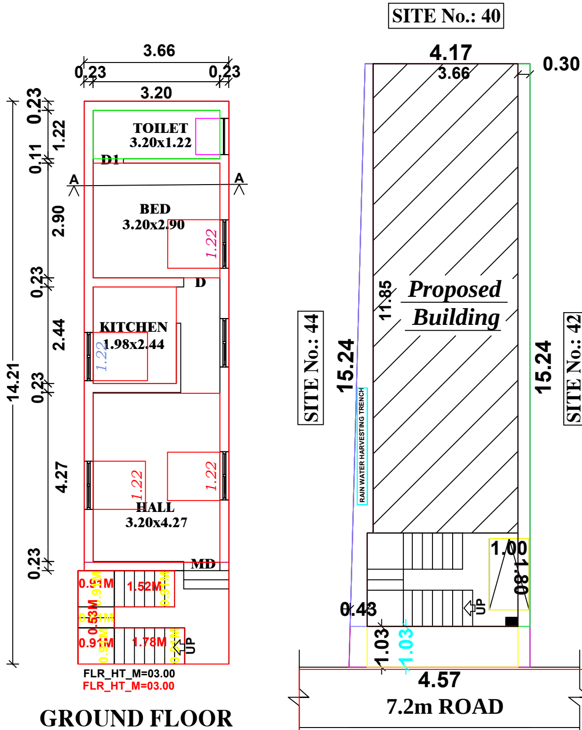
SITE PLAN
