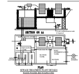
PLAN SEWAGE TREATMENT PLANT DETAILS WATER WATER RECIRCULATION
