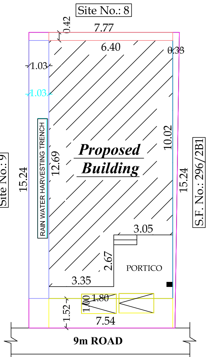
SITE PLAN
