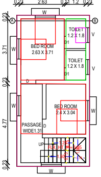
PROPOSED FIRST FLOOR BUILDING
