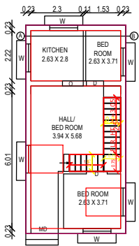
PROPOSED GROUND FLOOR BUILDING
