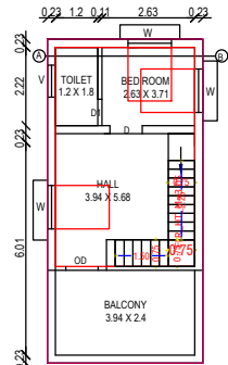
PROPOSED FIRST FLOOR BUILDING
