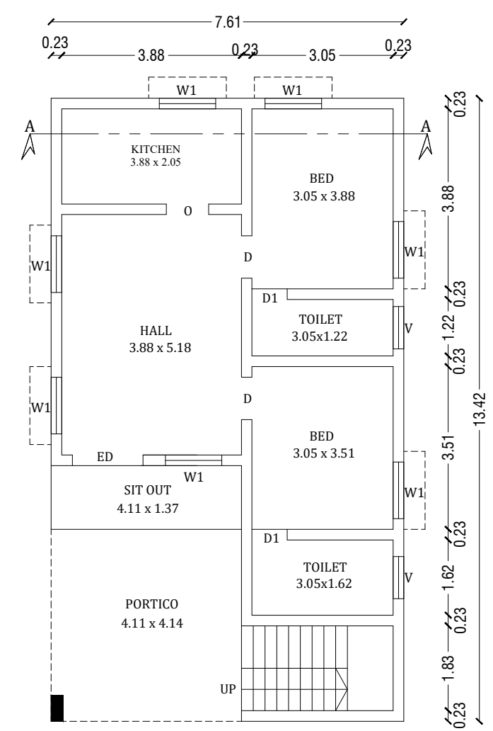
EXI. GROUND FLOOR PLAN
