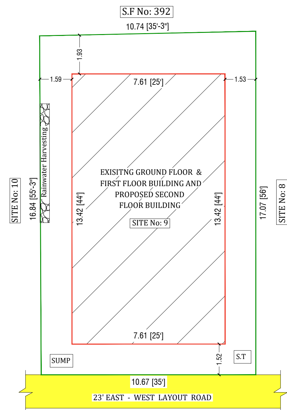
SITE PLAN
