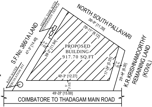
SITE PLAN SITE AREA - 1340.00 SQ.FT
