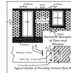
Sectional Elevation of Door and Window
