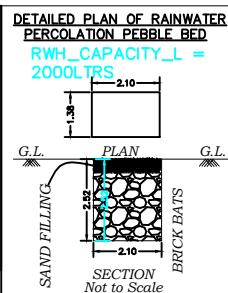
SECTION Not to Scale
