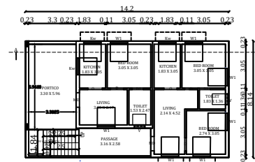
EXISTING GROUND FLOOR PLAN
