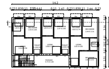
PROPOSED FIRST FLOOR PLAN
