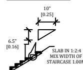
STAIR CASE DETAILS :-
