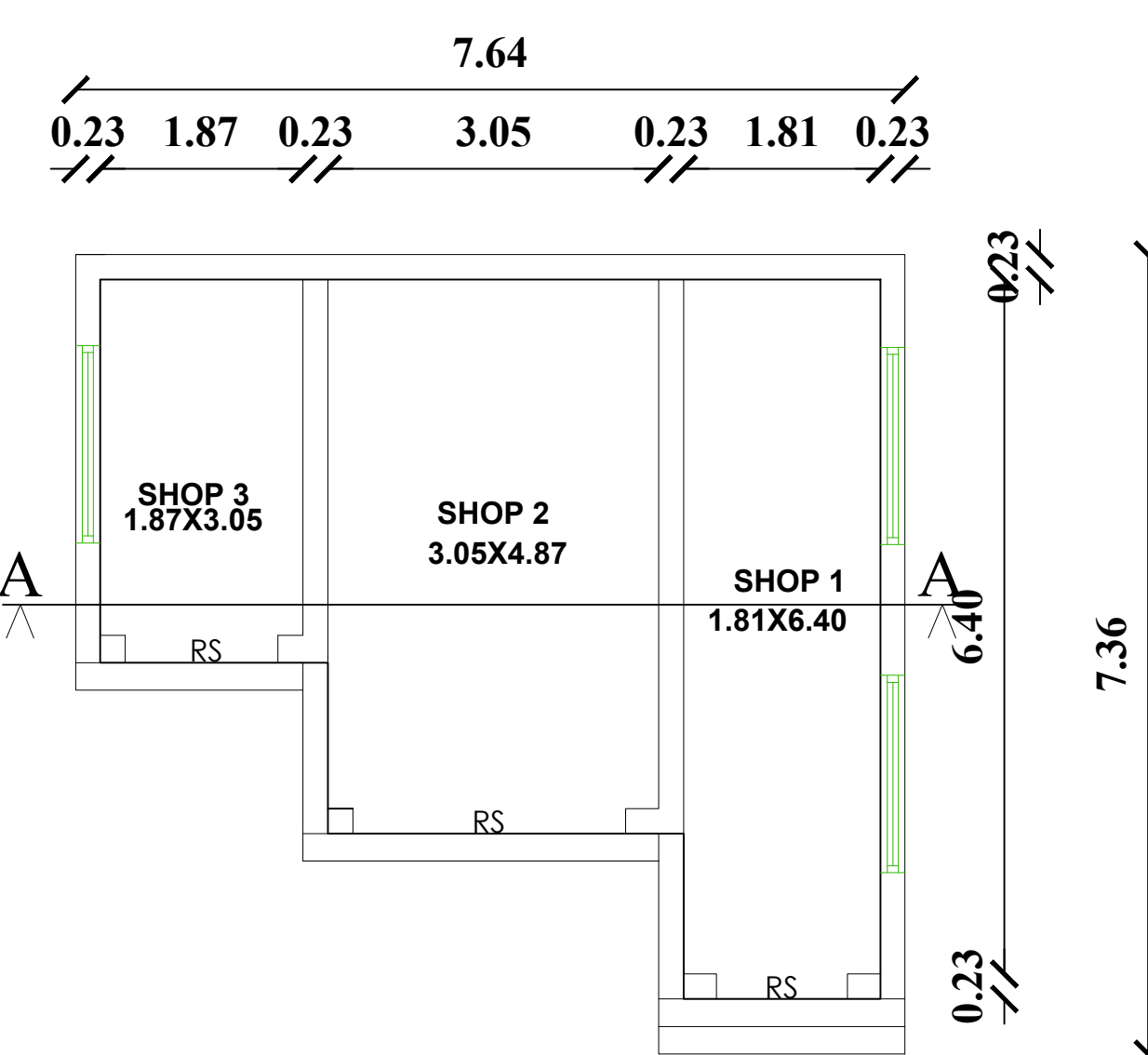
PRO.SHOP PLAN
