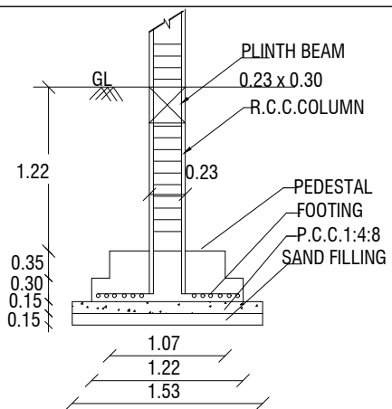
FOUNDATION DETAIL
