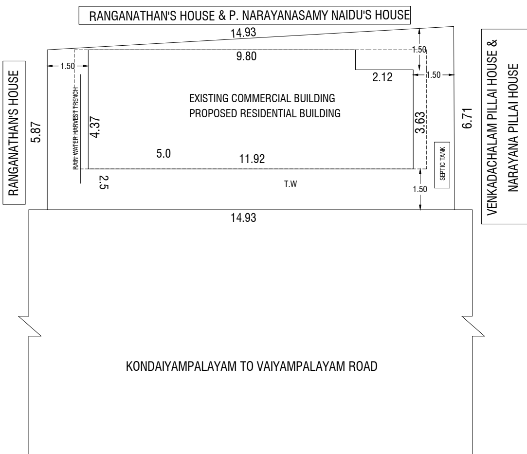
SITE PLAN
