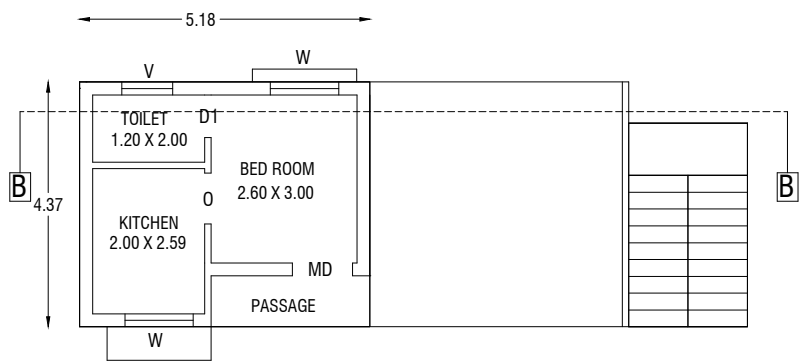
PROPOSED SECOND FLOOR PLAN
