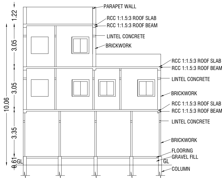
SECTION BB
