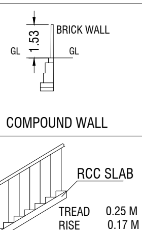
STAIRCASE DETAIL
